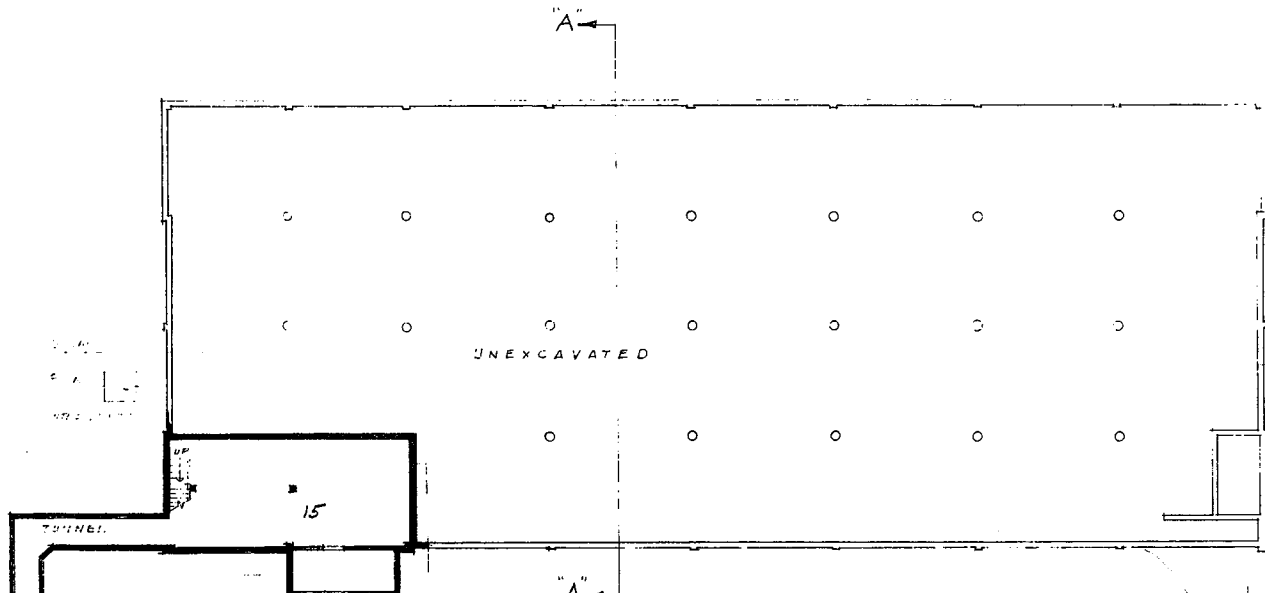
BASEMENT & FOUNDATION PLAN
